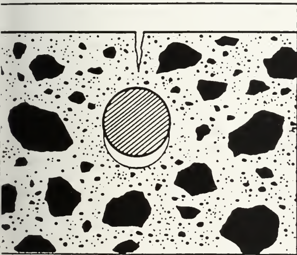
1.2—Crack formed due to obstructed settlement (Reference 2)
